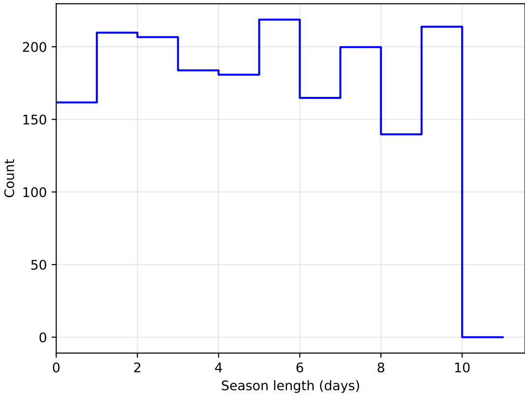
weather_cloudso10v3.4_10yrs DD:WFD all bands: SeasonLength
