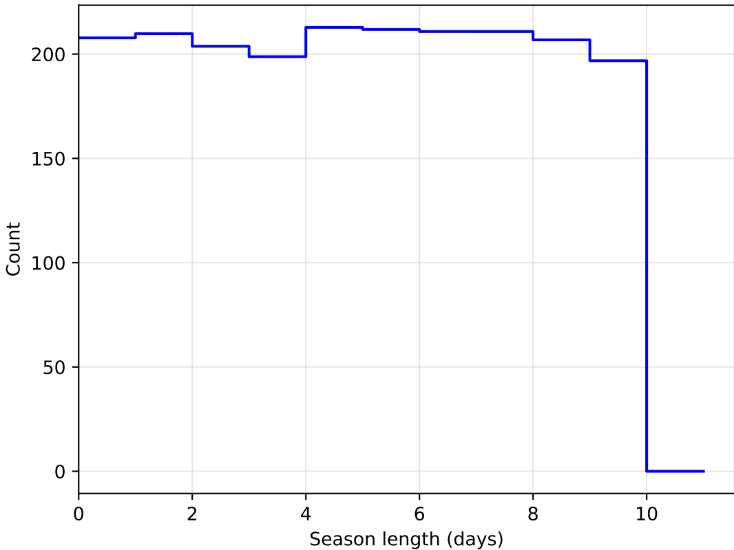
weather_cloudso10v3.4_10yrs DD:EDFS all bands: SeasonLength
