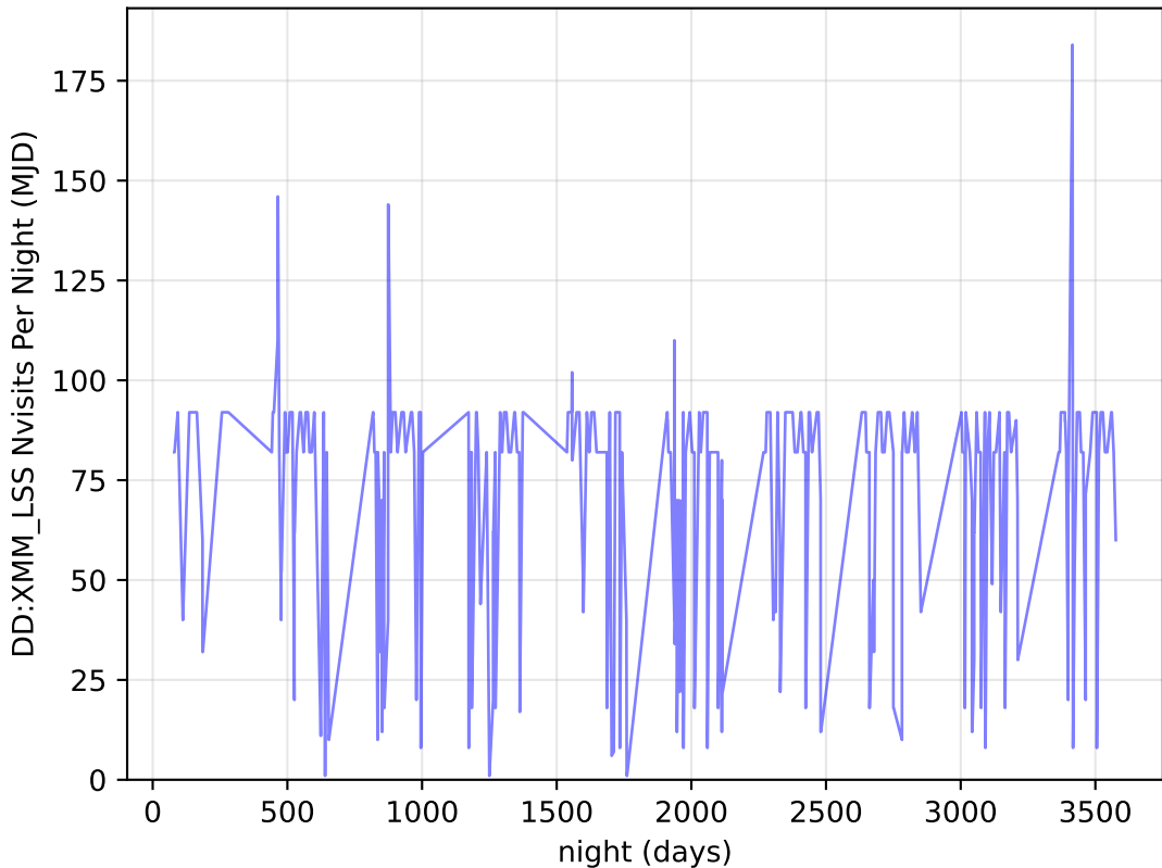
weather_cloudso10v3.4_10yrs all bands: DD:XMM_LSS Nvisits Per Night
