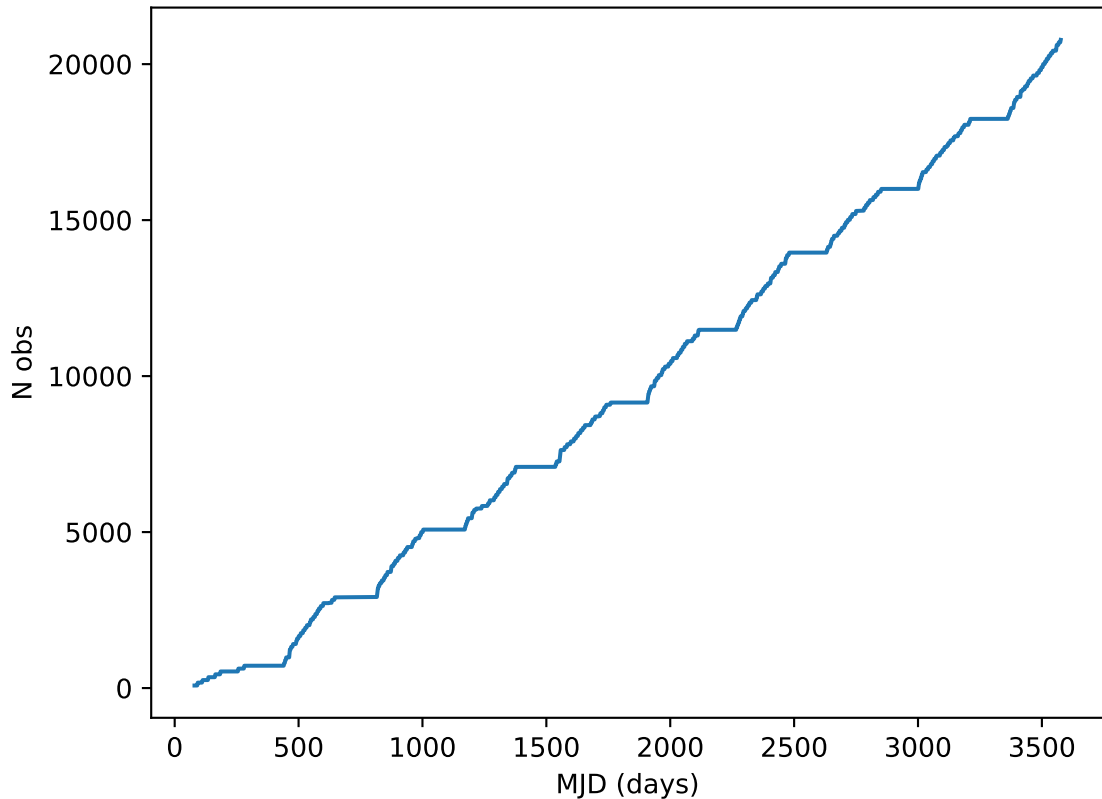
weather_cloudso10v3.4_10yrs all bands: DD:XMM_LSS Cumulative NVisits
