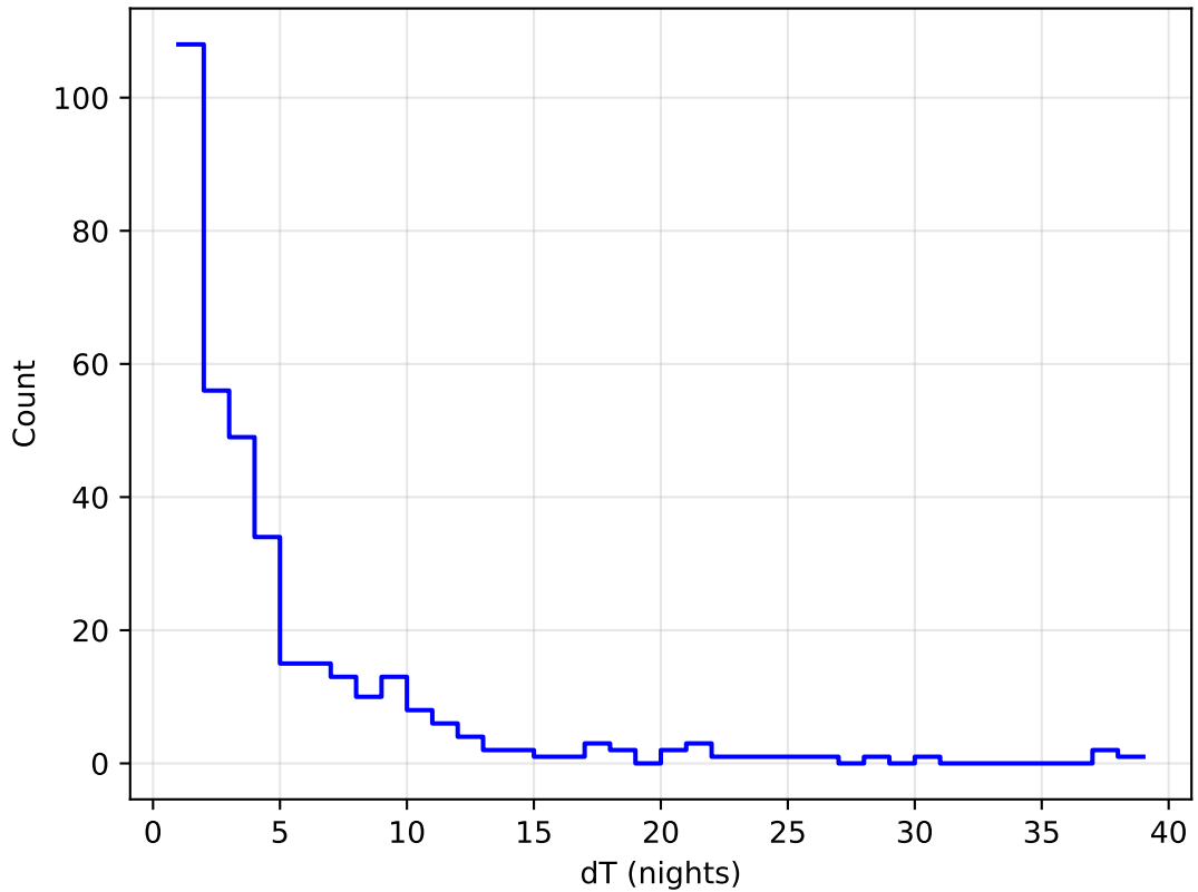
weather_cloudso10v3.4_10yrs all bands: DD:WFD Delta Nights Histogram
