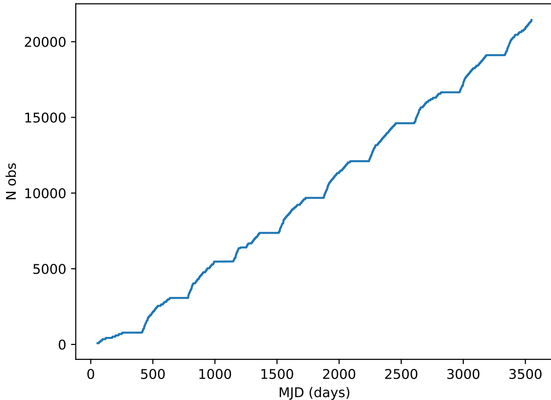
weather_cloudso10v3.4_10yrs all bands: DD:ELAISS1 Cumulative NVisits
