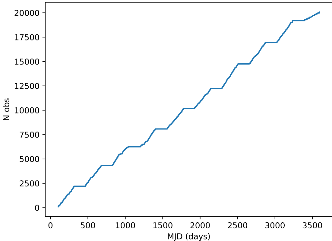
weather_cloudso10v3.4_10yrs all bands: DD:EDFS Cumulative NVisits
