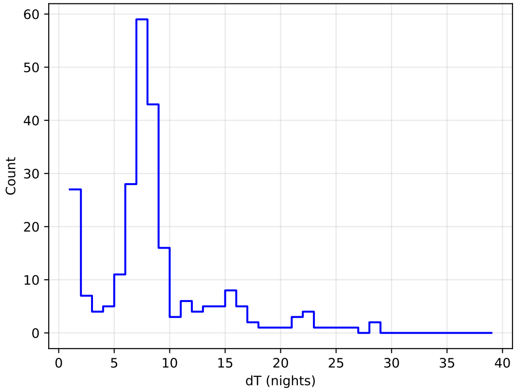
weather_cloudso10v3.4_10yrs all bands: DD:ECDFS Delta Nights Histogram
