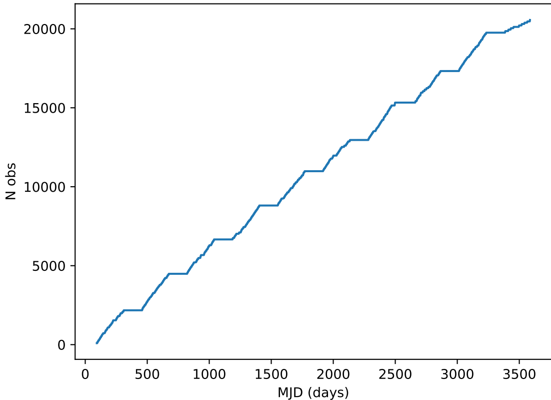
weather_cloudso10v3.4_10yrs all bands: DD:ECDFS Cumulative NVisits
