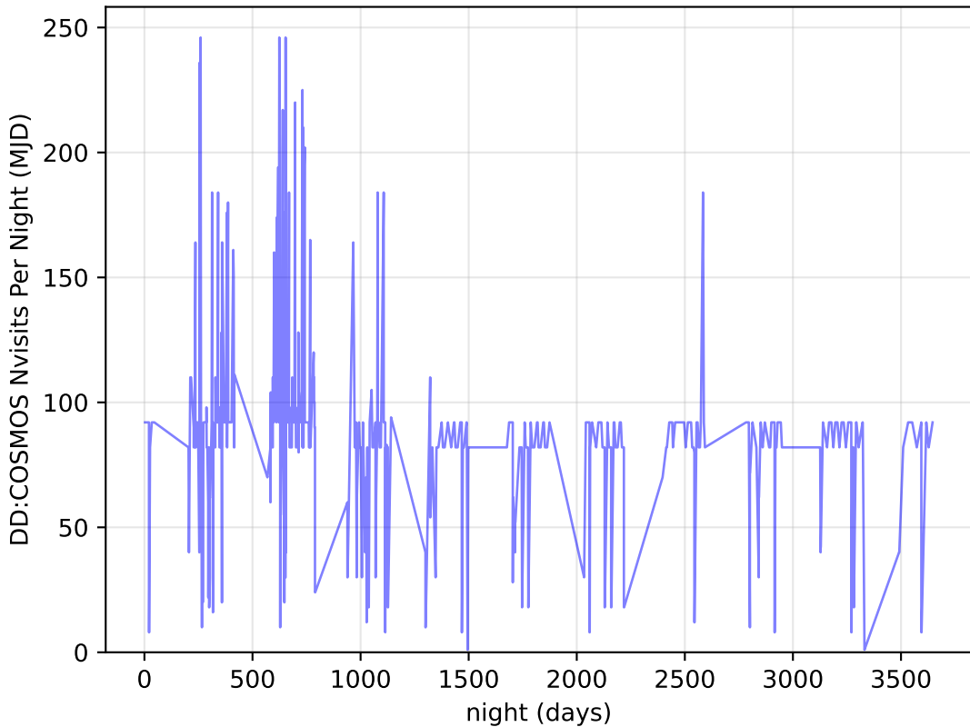
weather_cloudso10v3.4_10yrs all bands: DD: COSMOS Nvisits Per Night
