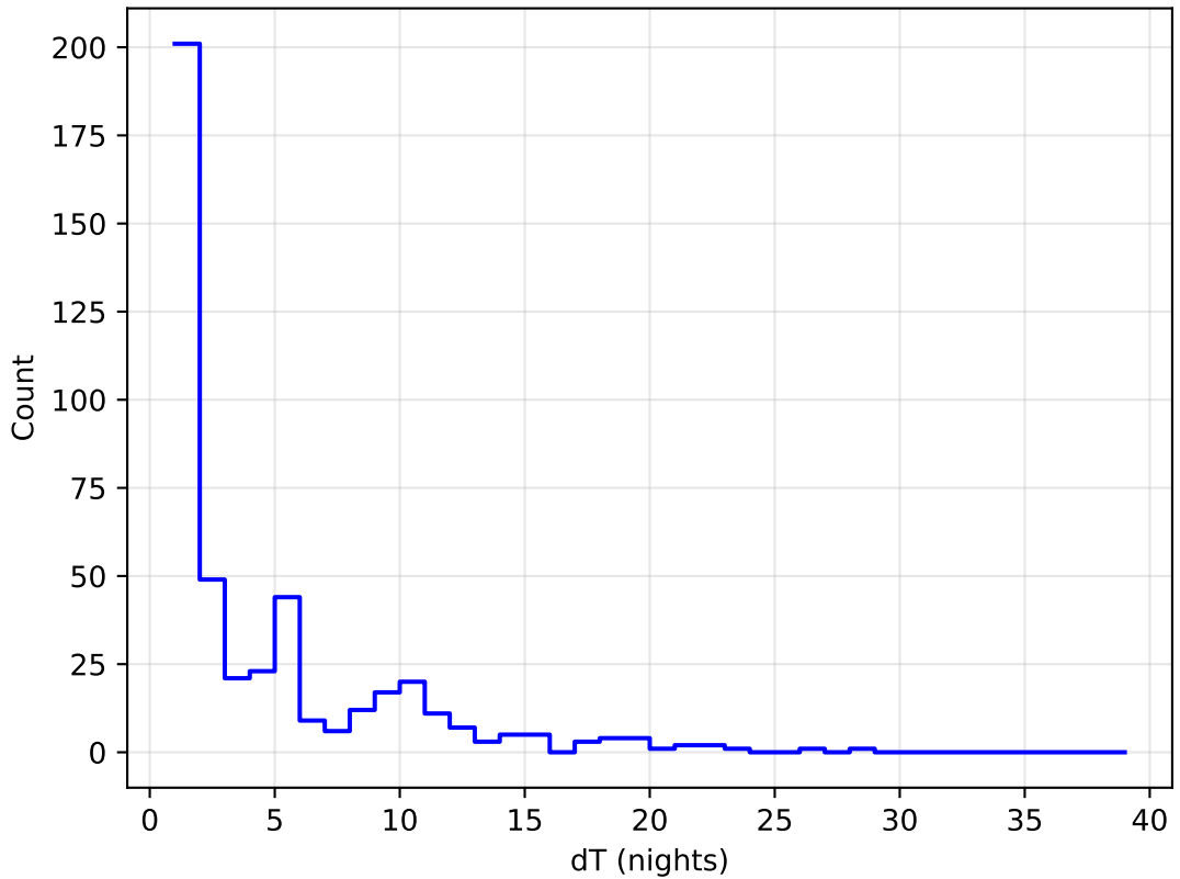
weather_cloudso10v3.4_10yrs all bands: DD: COSMOS Delta Nights Histogram
