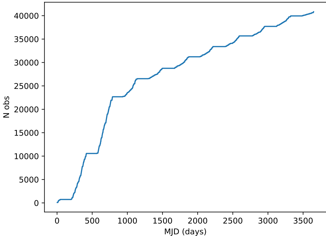
weather_cloudso10v3.4_10yrs all bands: DD:COSMOS Cumulative NVisits
