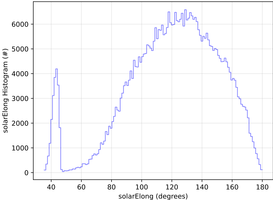
weather_cloudso0v3.5_10yrs WFD z band: solarElong Histogram
