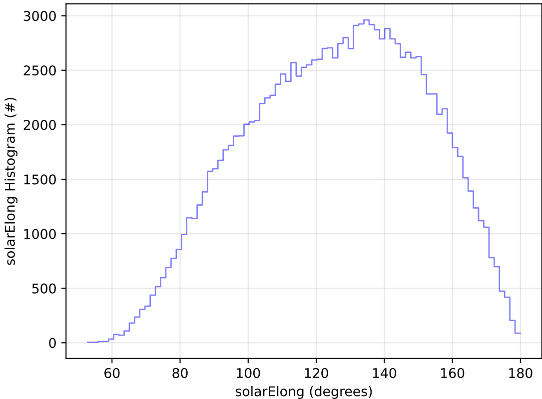
weather_cloudso0v3.5_10yrs WFD u band: solarElong Histogram
