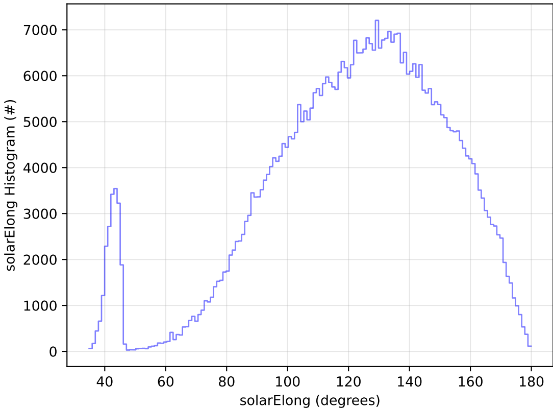
weather_cloudso0v3.5_10yrs WFD r band: solarElong Histogram
