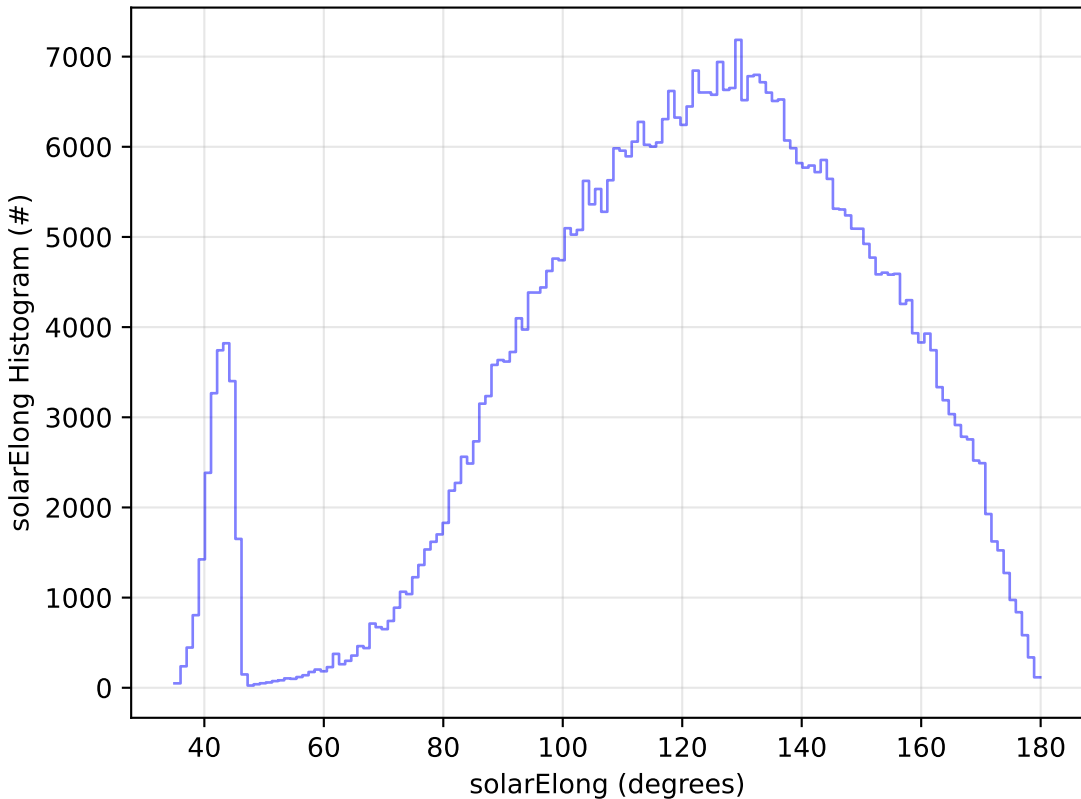
weather_cloudso0v3.5_10yrs WFD i band: solarElong Histogram
