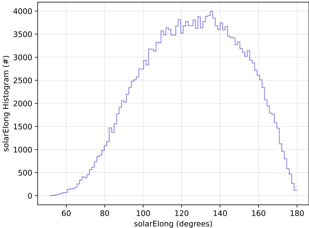
weather_cloudso0v3.5_10yrs WFD g band: solarElong Histogram
