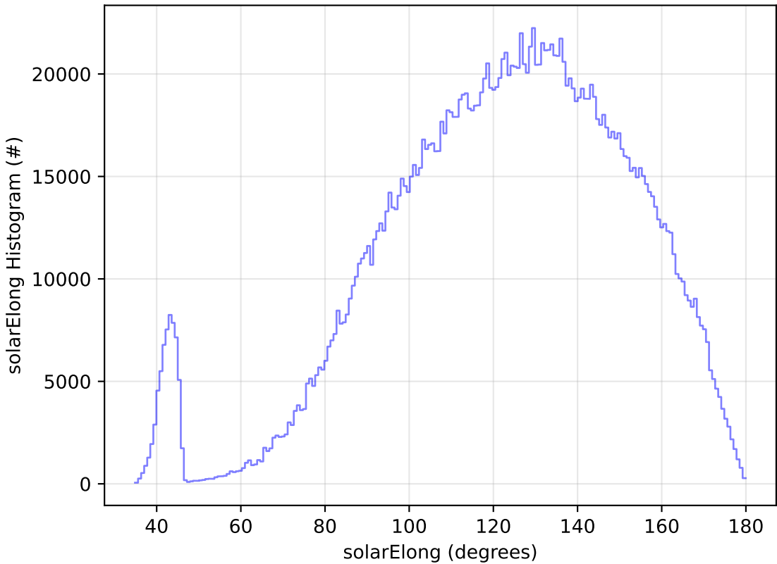
weather_cloudso0v3.5_10yrs WFD all bands: solarElong Histogram
