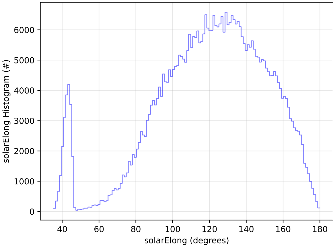
weather_cloudso0v3.5_10yrs All sky z band: solarElong Histogram
