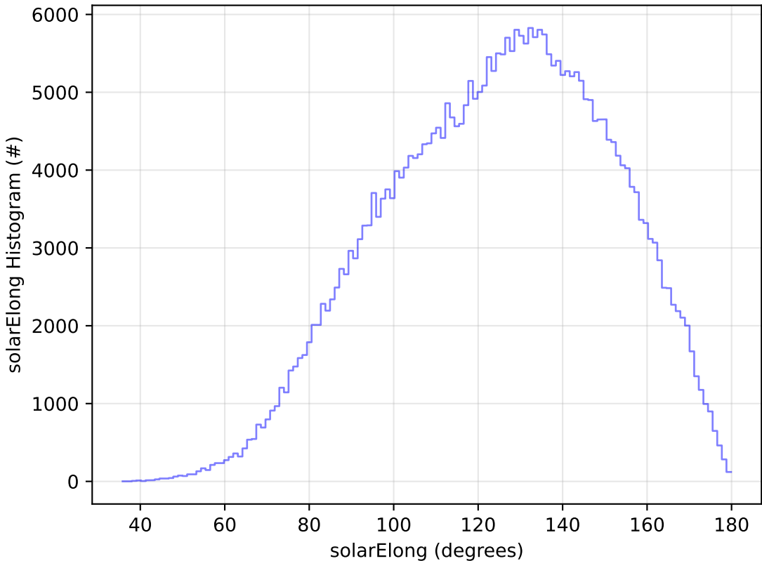
weather_cloudso0v3.5_10yrs All sky y band: solarElong Histogram
