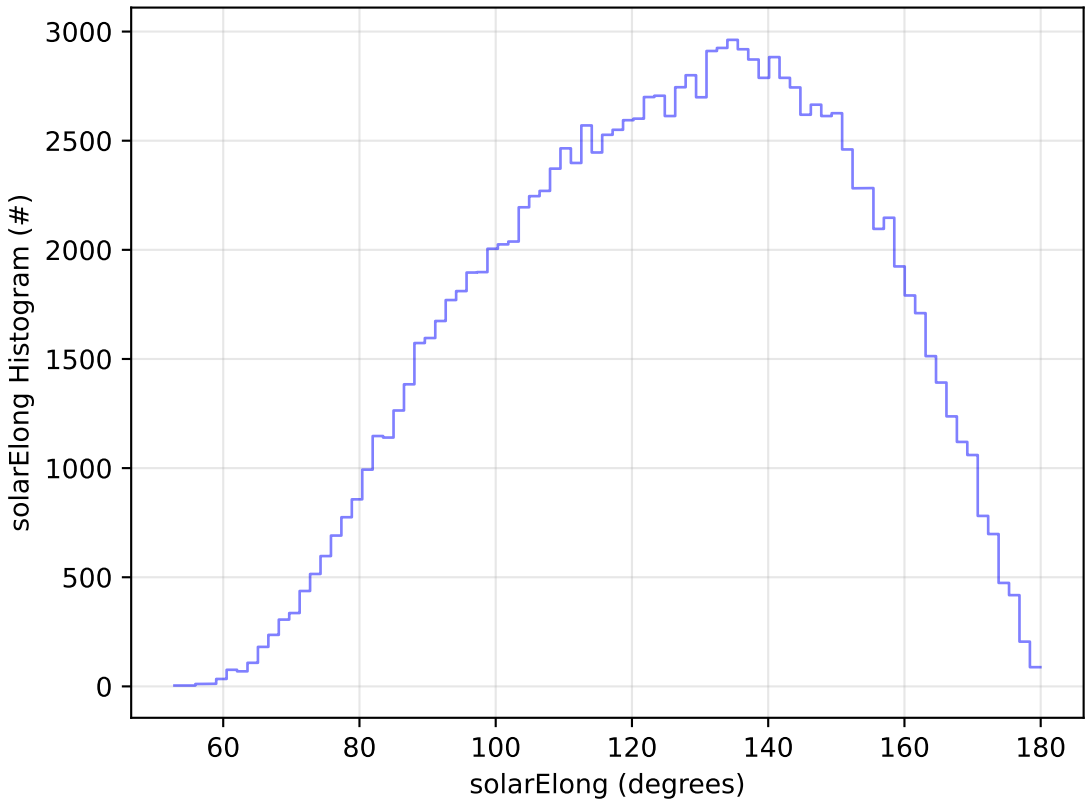
weather_cloudso0v3.5_10yrs All sky u band: solarElong Histogram
