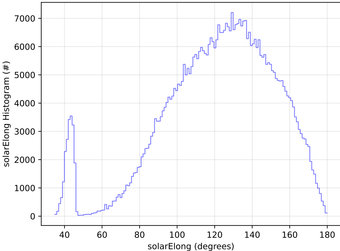
weather_cloudso0v3.5_10yrs All sky r band: solarElong Histogram
