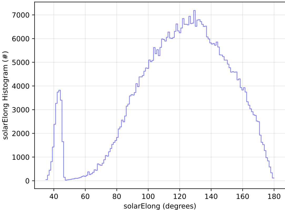
weather_cloudso0v3.5_10yrs All sky i band: solarElong Histogram
