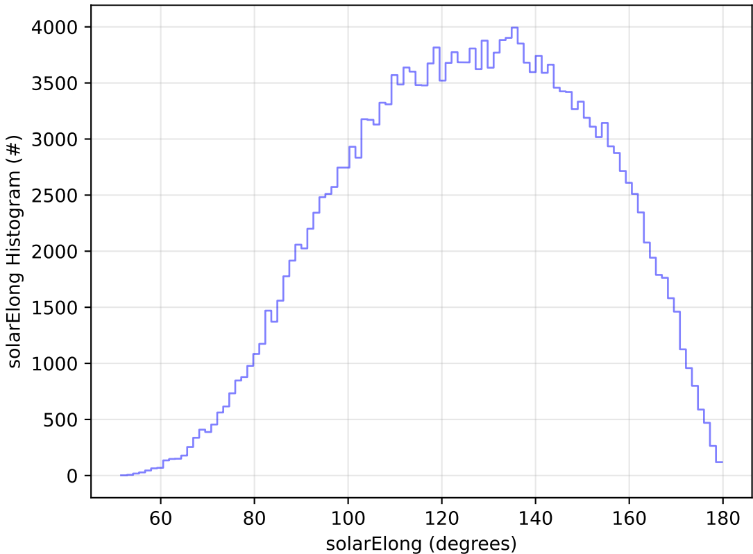
weather_cloudso0v3.5_10yrs All sky g band: solarElong Histogram
