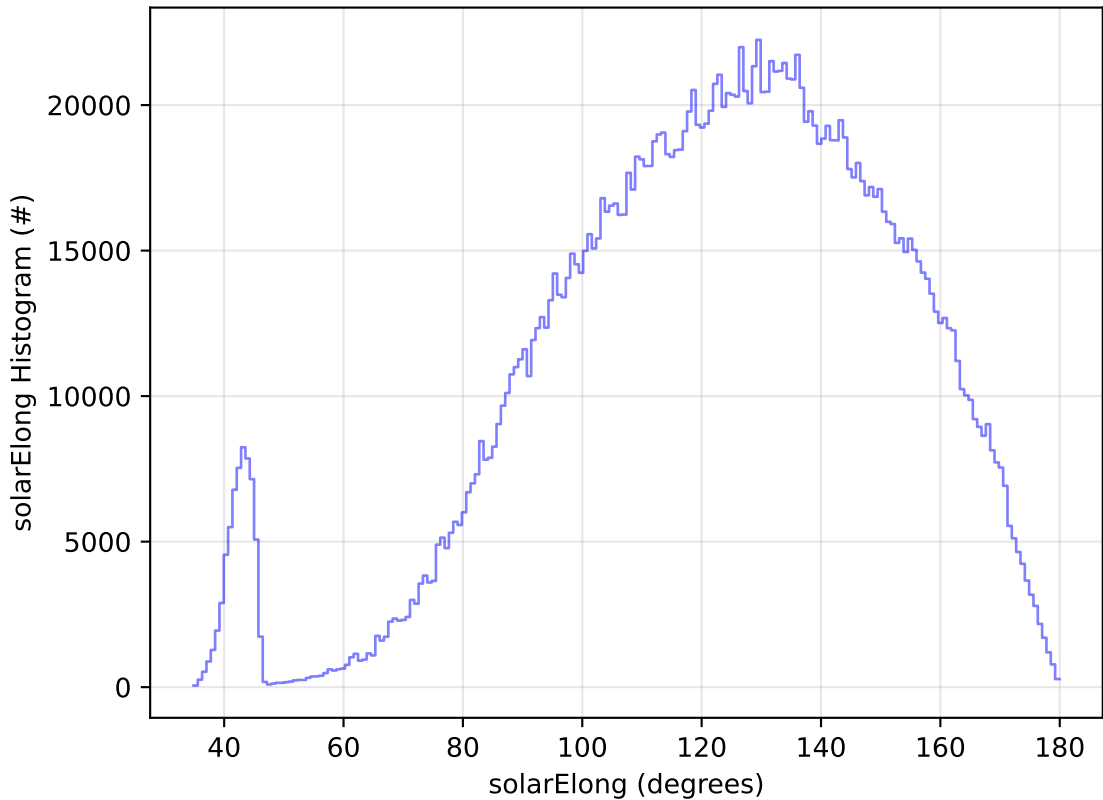
weather_cloudso0v3.5_10yrs All sky all bands: solarElong Histogram
