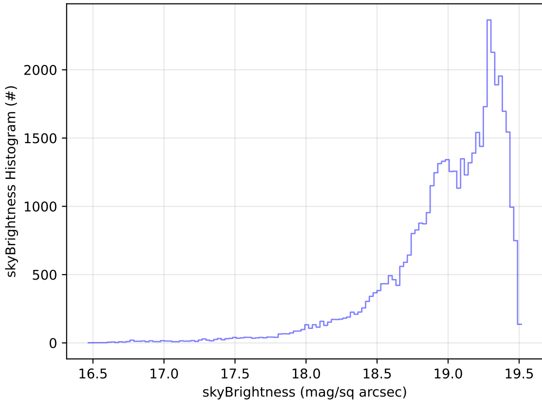
weather_cloudso0v3.5_10yrs Yr 1 z band: skyBrightness Histogram
