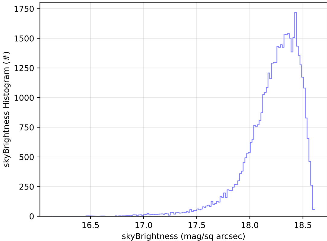
weather_cloudso0v3.5_10yrs Yr 1 y band: skyBrightness Histogram
