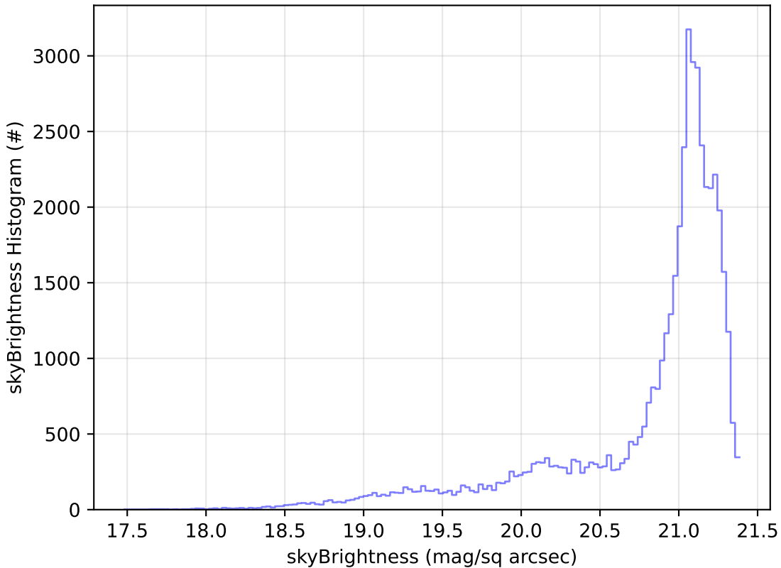
weather_cloudso0v3.5_10yrs Yr 1 r band: skyBrightness Histogram
