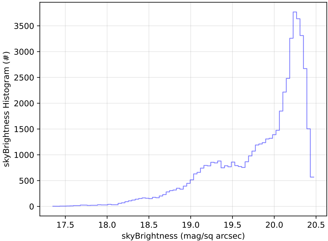
weather_cloudso0v3.5_10yrs Yr 1 i band: skyBrightness Histogram
