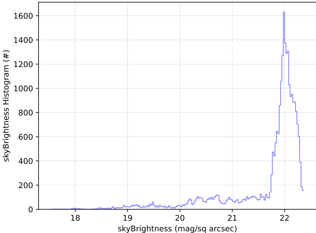
weather_cloudso0v3.5_10yrs Yr 1 g band: skyBrightness Histogram
