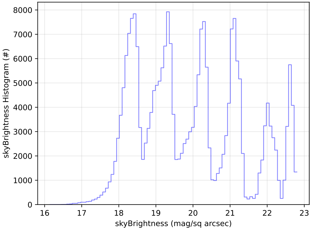
weather_cloudso0v3.5_10yrs Yr 1 all bands: skyBrightness Histogram
