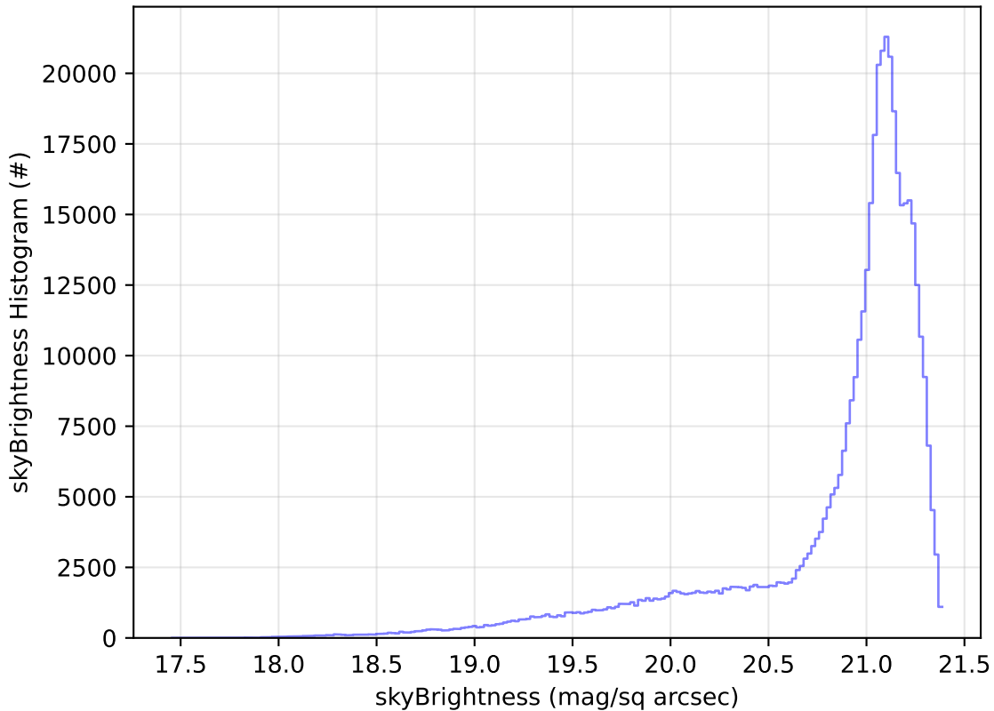
weather_cloudso0v3.5_10yrs WFD r band: skyBrightness Histogram
