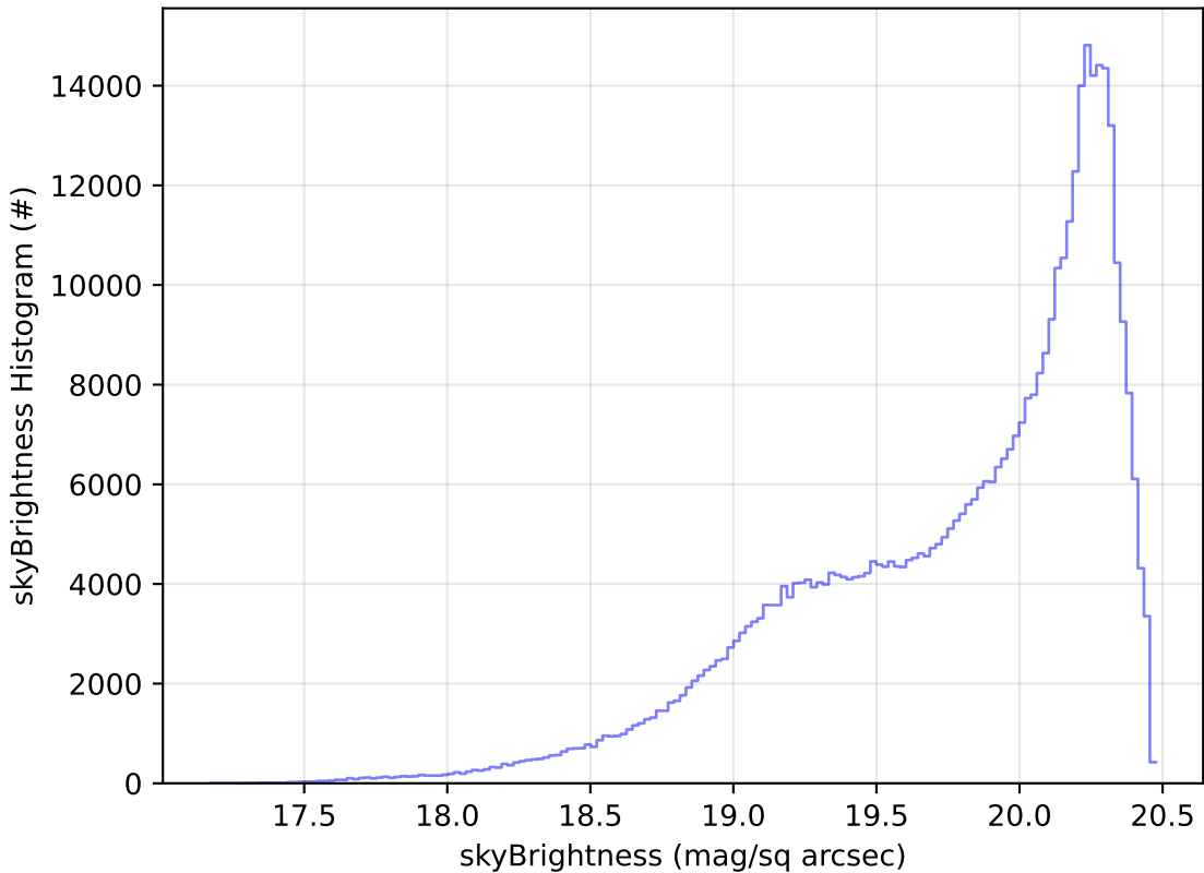
weather_cloudso0v3.5_10yrs WFD i band: skyBrightness Histogram
