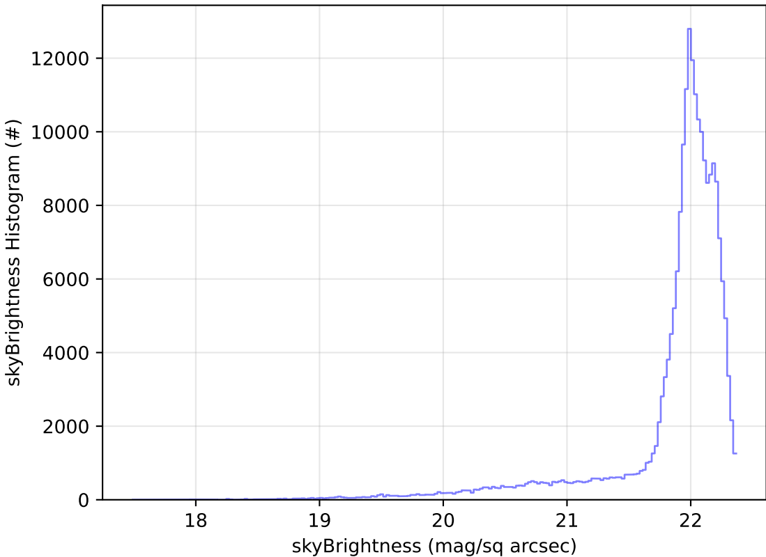
weather_cloudso0v3.5_10yrs WFD g band: skyBrightness Histogram
