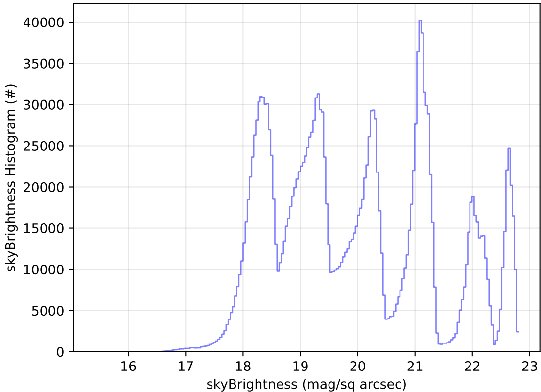
weather_cloudso0v3.5_10yrs WFD all bands: skyBrightness Histogram
