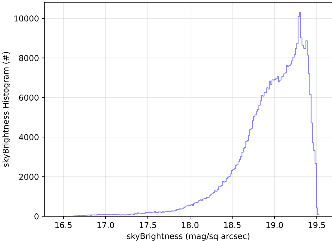
weather_cloudso0v3.5_10yrs All sky z band: skyBrightness Histogram
