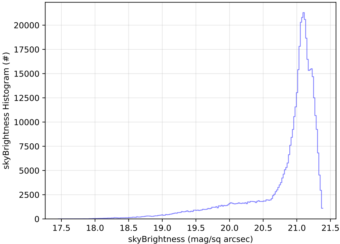
weather_cloudso0v3.5_10yrs All sky r band: skyBrightness Histogram
