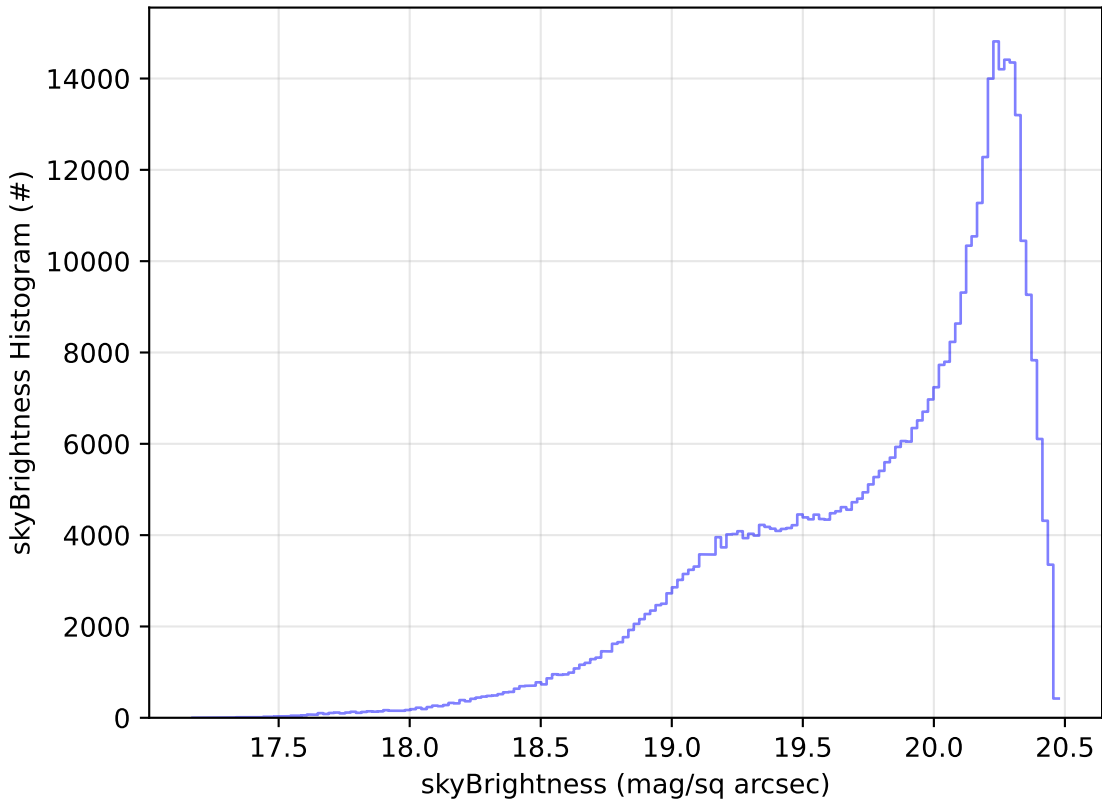
weather_cloudso0v3.5_10yrs All sky i band: skyBrightness Histogram
