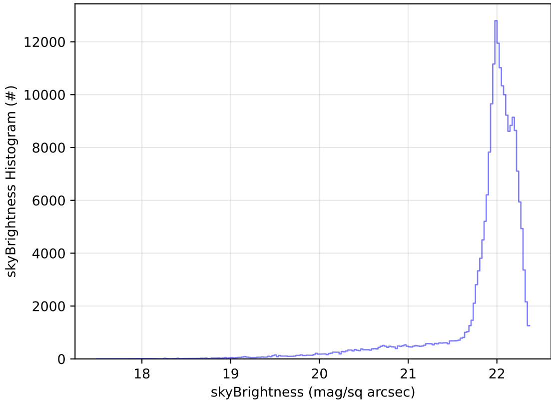
weather_cloudso0v3.5_10yrs All sky g band: skyBrightness Histogram
