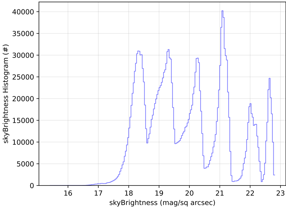
weather_cloudso0v3.5_10yrs All sky all bands: skyBrightness Histogram
