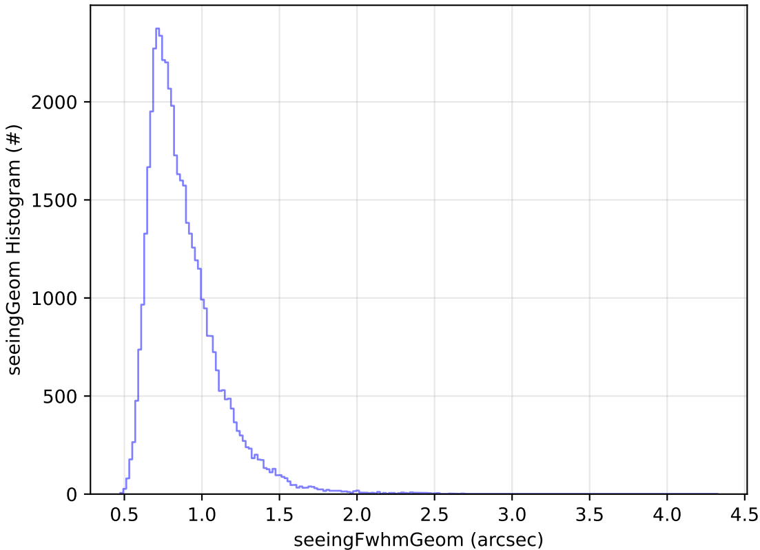
weather_cloudso0v3.5_10yrs Yr 1 z band: seeingGeom Histogram
