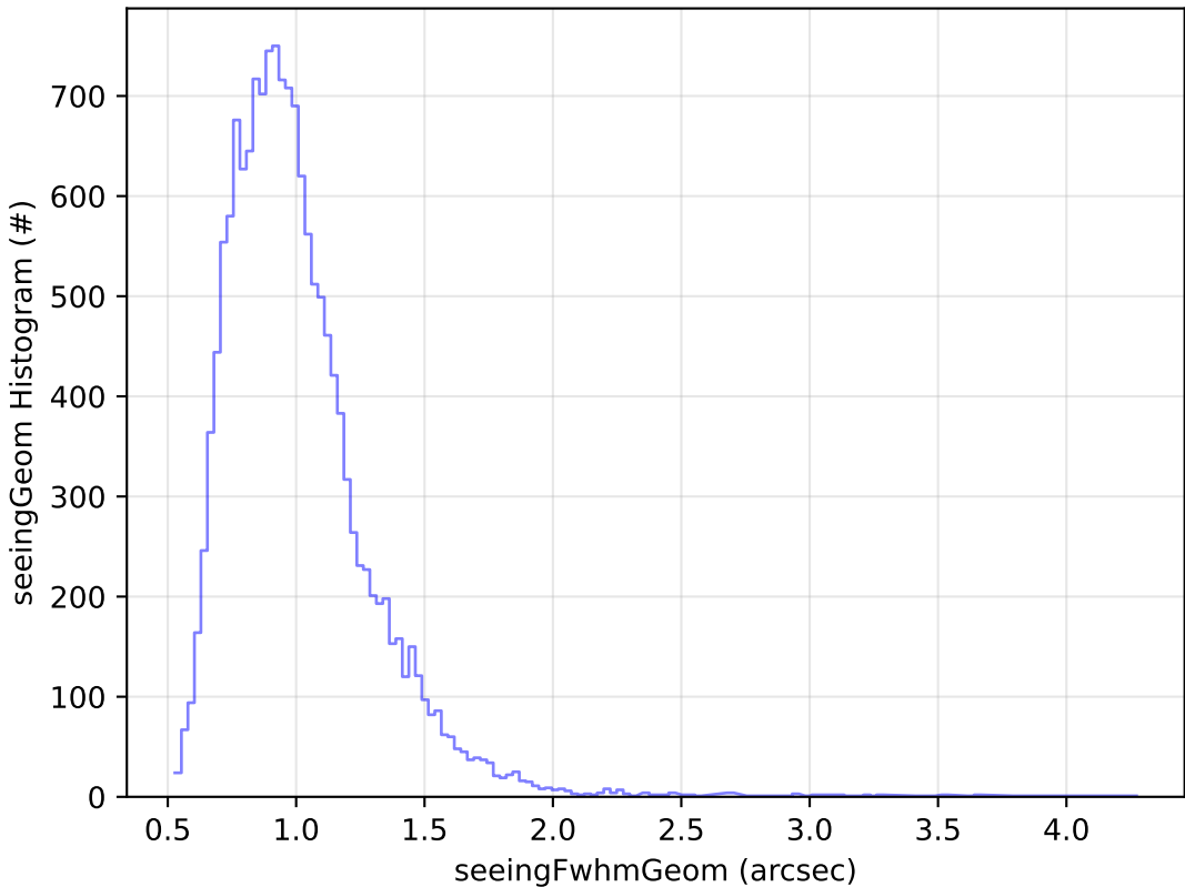
weather_cloudso0v3.5_10yrs Yr 1 u band: seeingGeom Histogram
