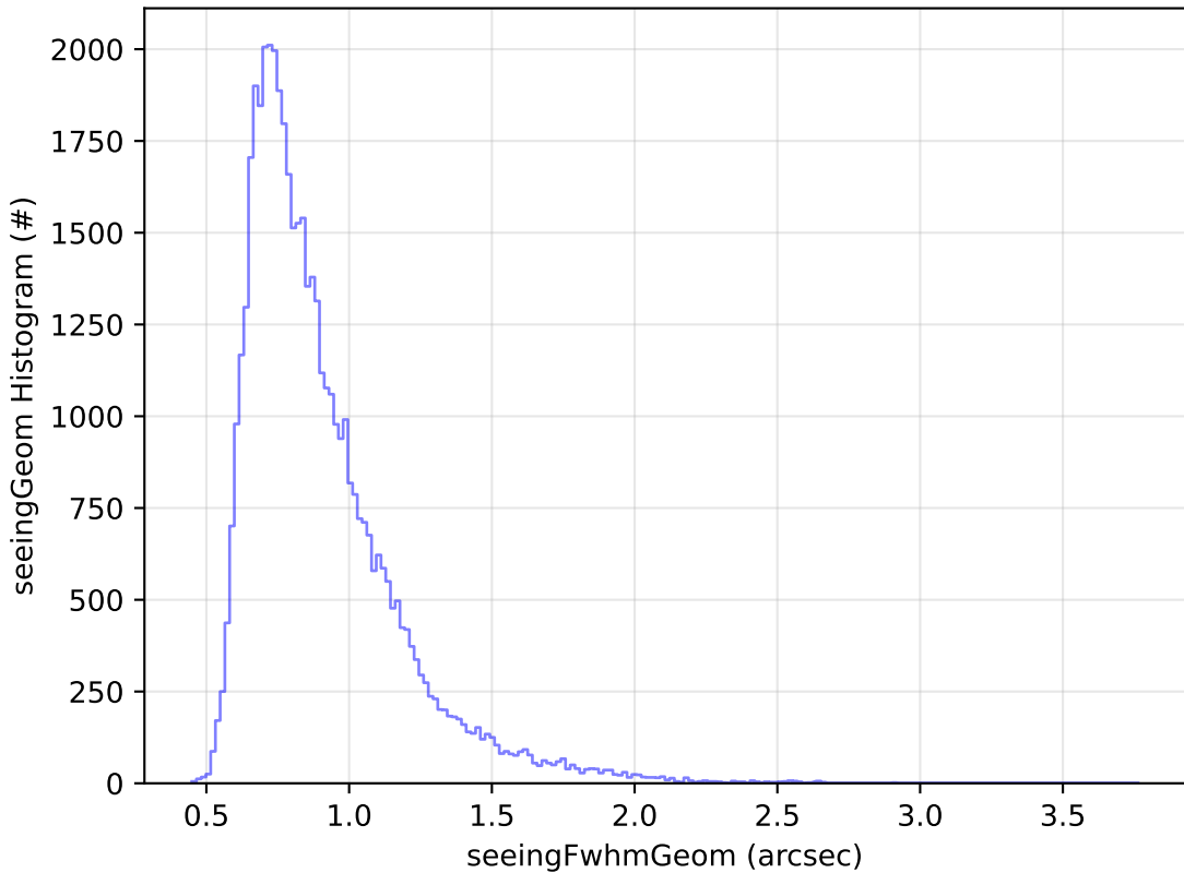
weather_cloudso0v3.5_10yrs Yr 1 r band: seeingGeom Histogram
