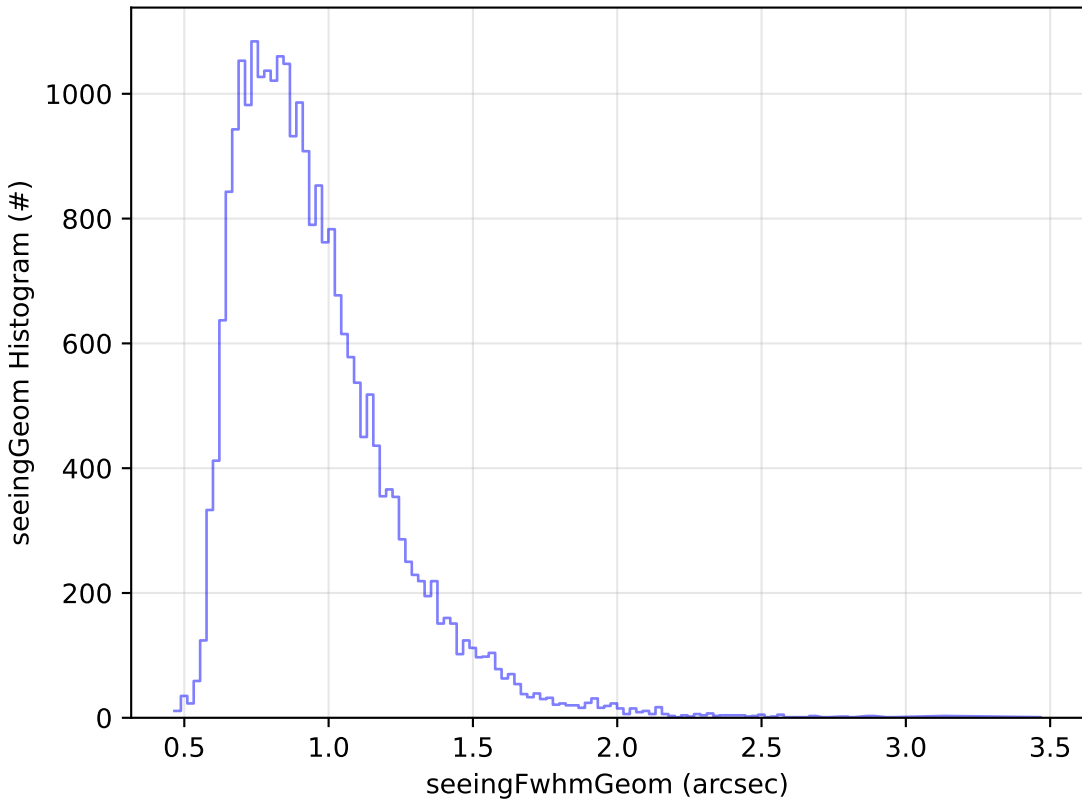
weather_cloudso0v3.5_10yrs Yr 1 g band: seeingGeom Histogram
