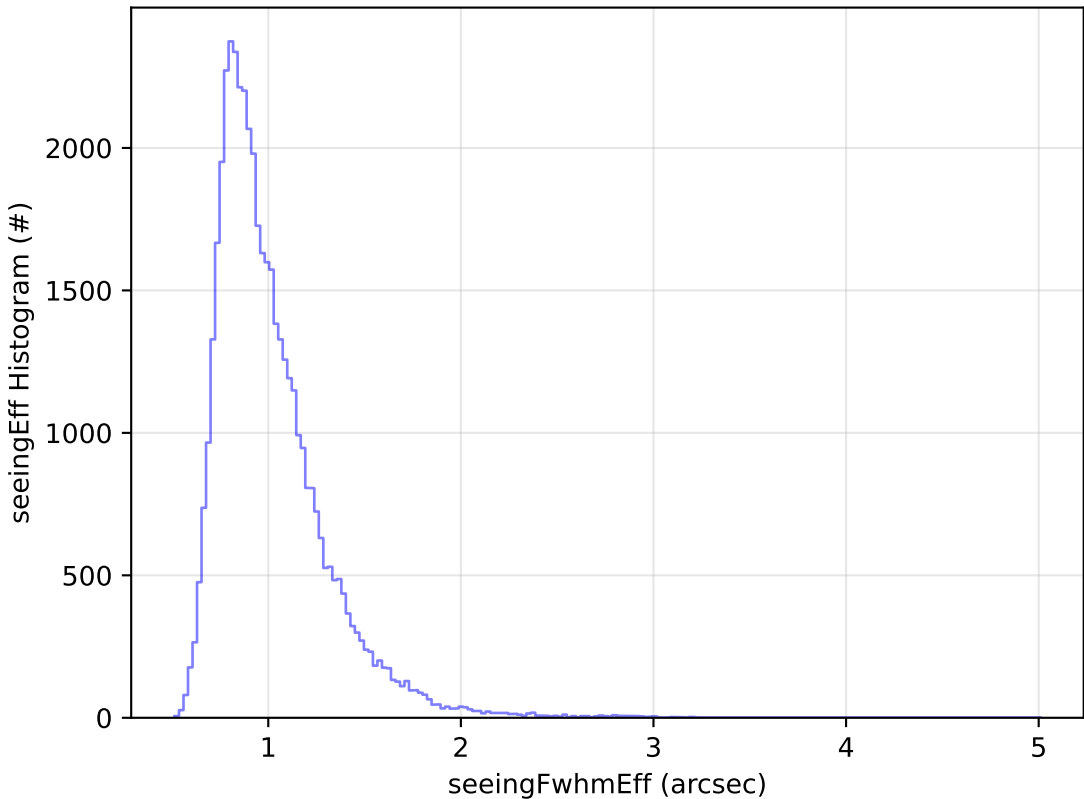
weather_cloudso0v3.5_10yrs Yr 1 z band: seeingEff Histogram
