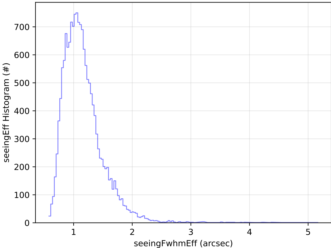
weather_cloudso0v3.5_10yrs Yr 1 u band: seeingEff Histogram
