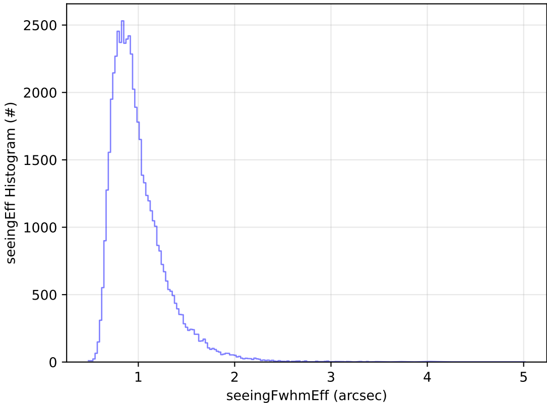
weather_cloudso0v3.5_10yrs Yr 1 i band: seeingEff Histogram
