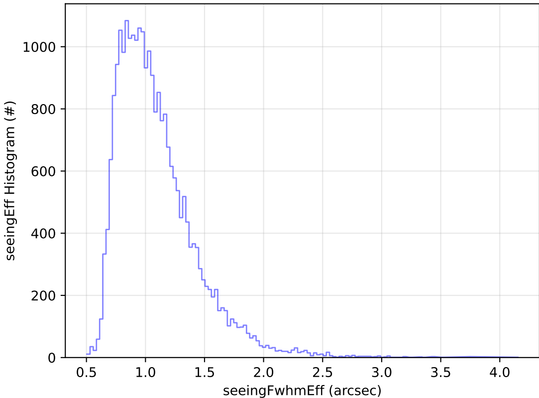
weather_cloudso0v3.5_10yrs Yr 1 g band: seeingEff Histogram
