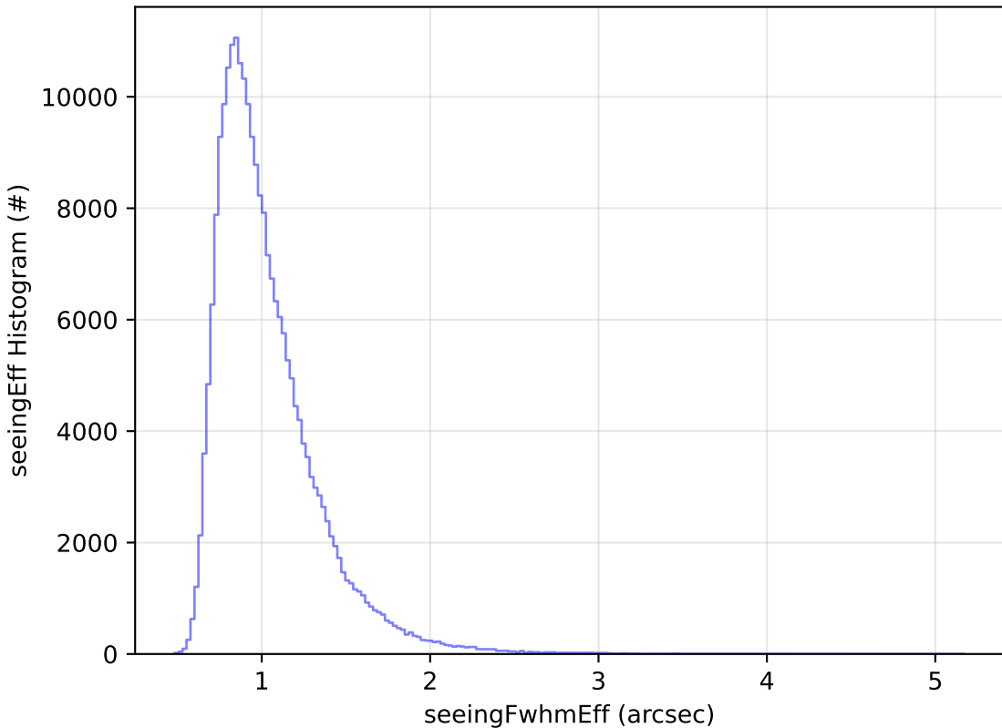
weather_cloudso0v3.5_10yrs Yr 1 all bands: seeingEff Histogram
