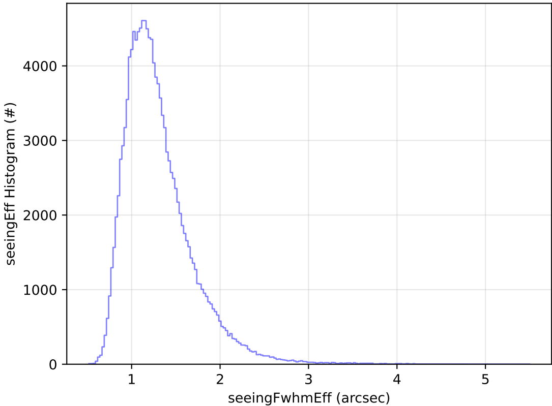
weather_cloudso0v3.5_10yrs WFD u band: seeingEff Histogram
